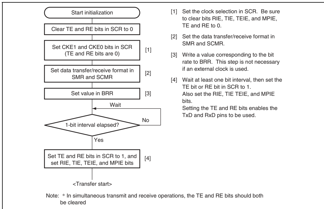
Figure 12.15 Sample SCI Initialization Flowchart
